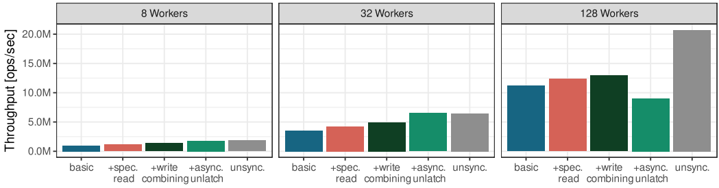
Fig. 9. Multi-threaded performance of optimized latches (4 compute nodes and 1 storage node).
