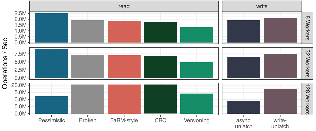
Fig. 15. Read-only and write-only optimistic scalability (4 compute nodes and 1 storage node).
